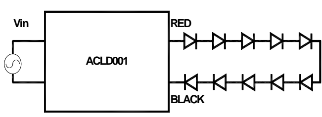
Application Wiring diagram
